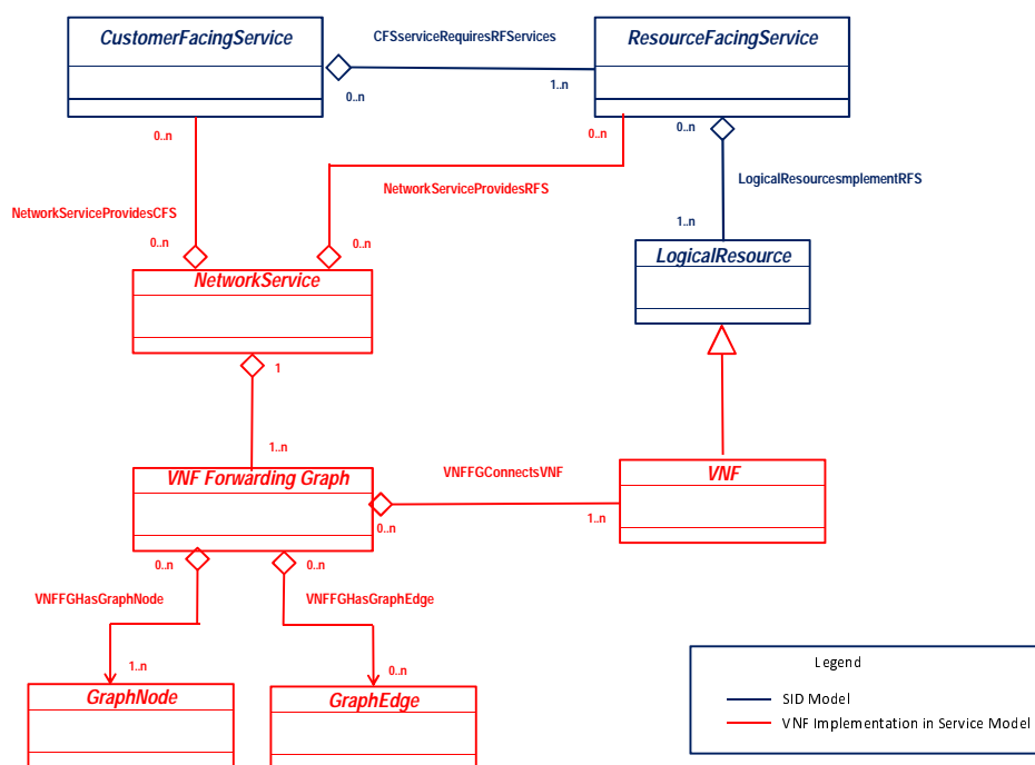
Figure G.3: VNF Implementation in SID Service Model
