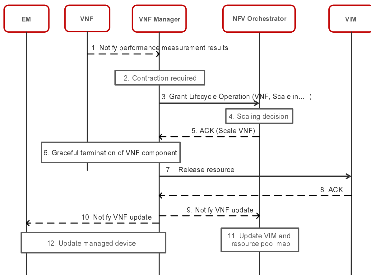
Figure B.15: Automatic VNF contraction flow triggered by VNF performance measurement results
