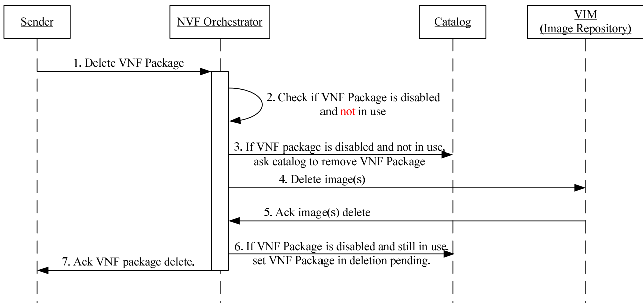
Figure B.7: Delete VNF Package message flow
