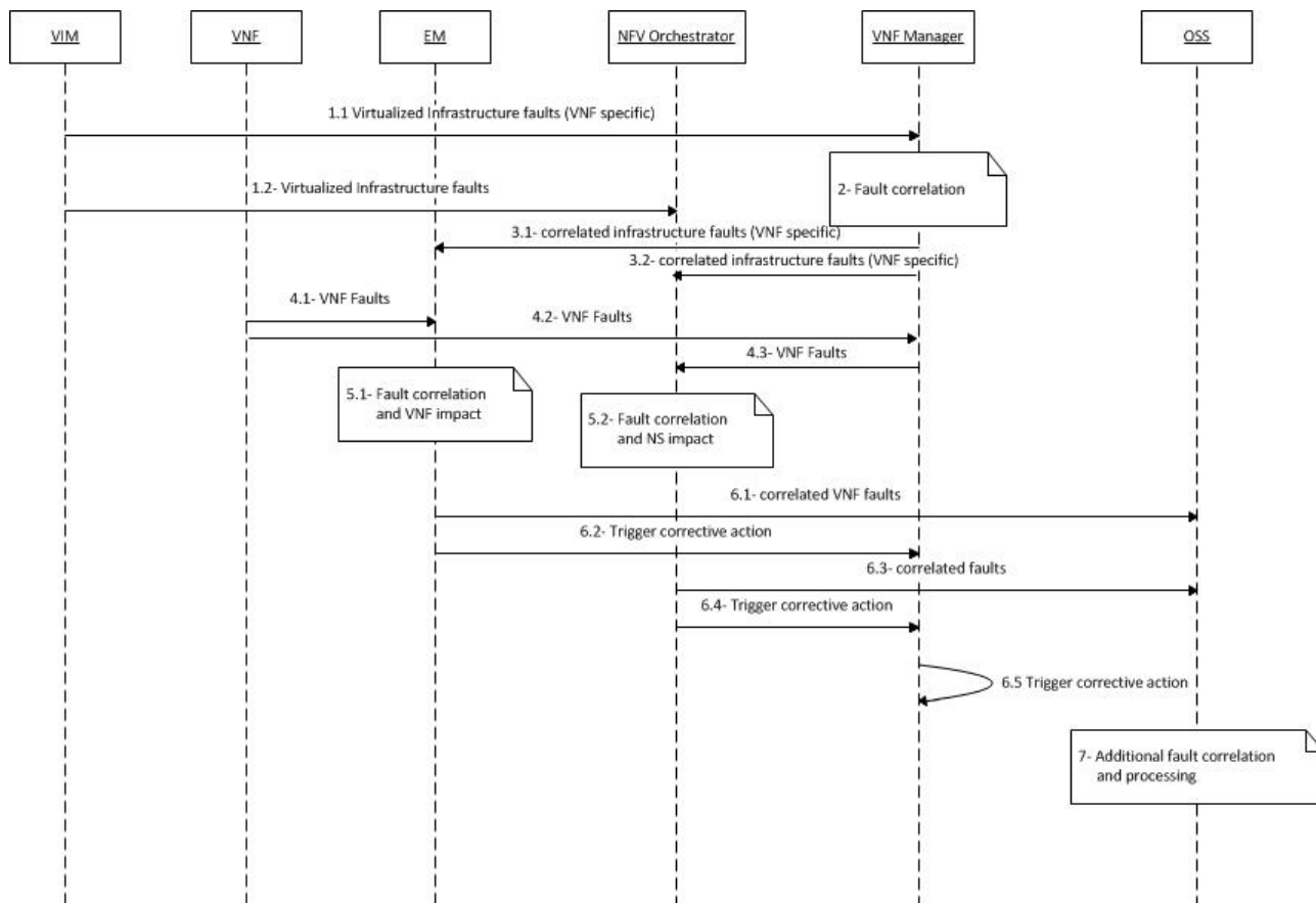
Figure B.18: NFV fault management flow
