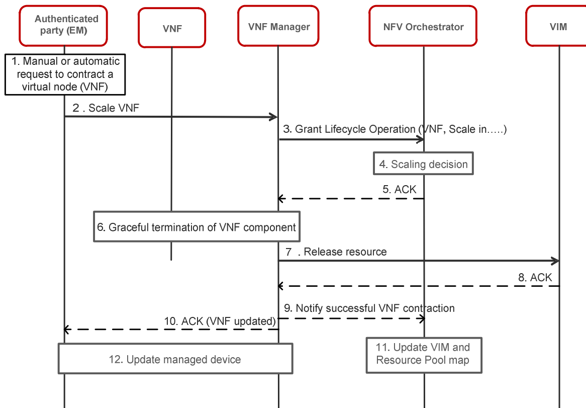
Figure B.16: EM initiated VNF contraction flow
