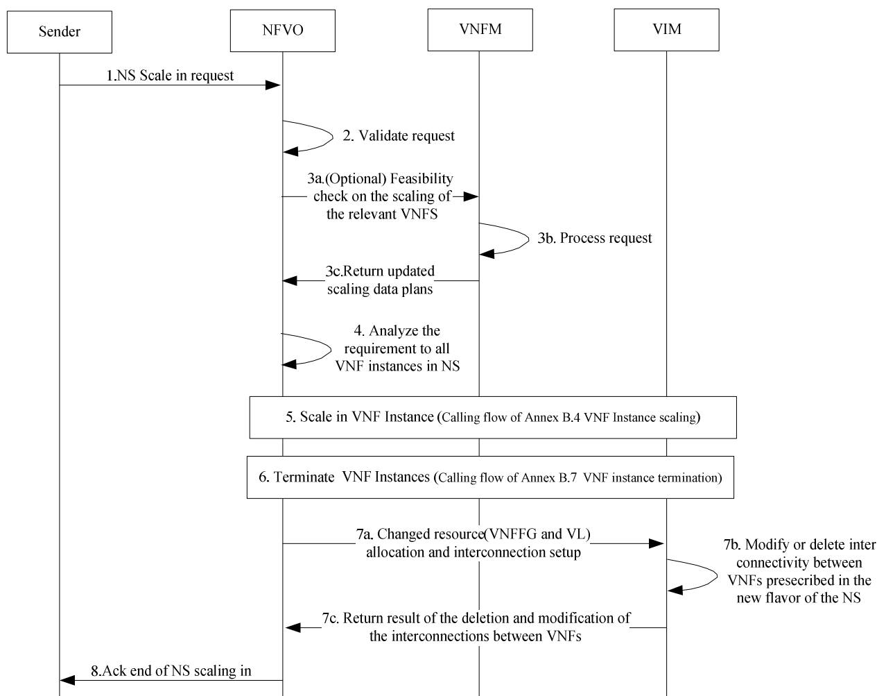
Figure C.10: Network Service scaling in message flow
