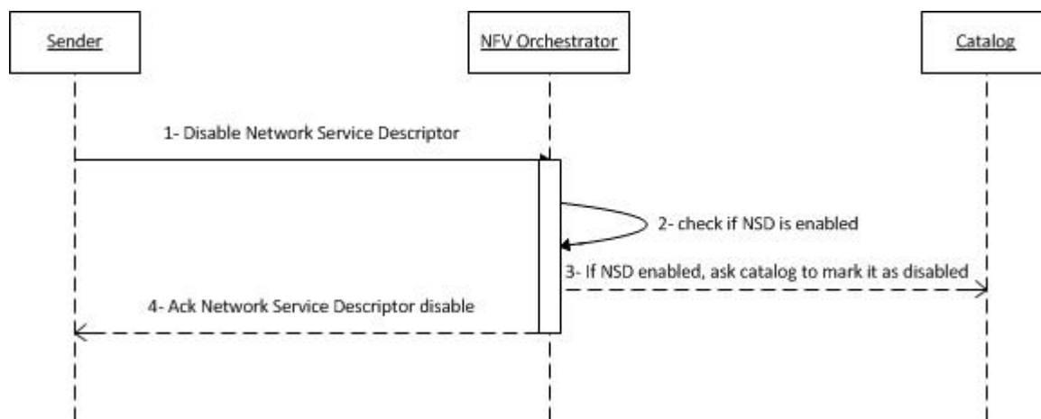
Figure C.3: Network Service Descriptor disable message flow
