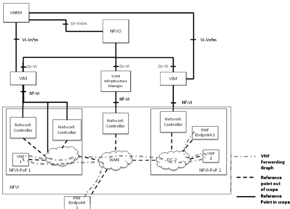
Figure 5.2: Network Controller example
