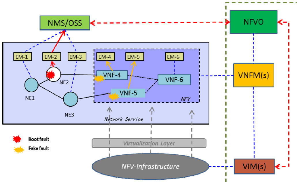
Figure A.8: Network Service fault
