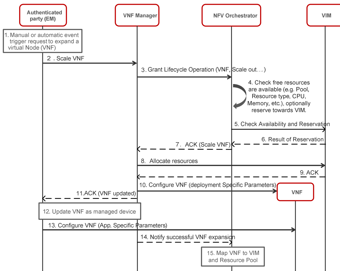
Figure B.14: EM initiated VNF expansion flow
