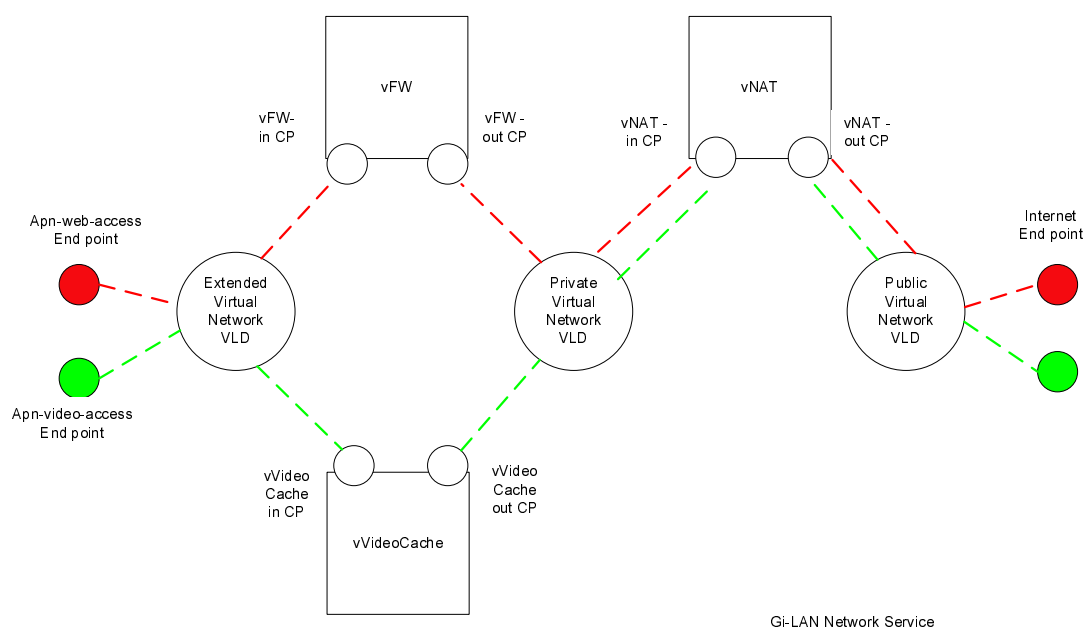
Figure F.1: Gi-LAN Network Service example used for modelling NSD and VNFD
