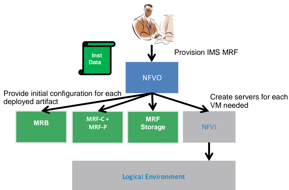
Figure A.4: IMS MRF VNF Forwarding Graph deployment use case
