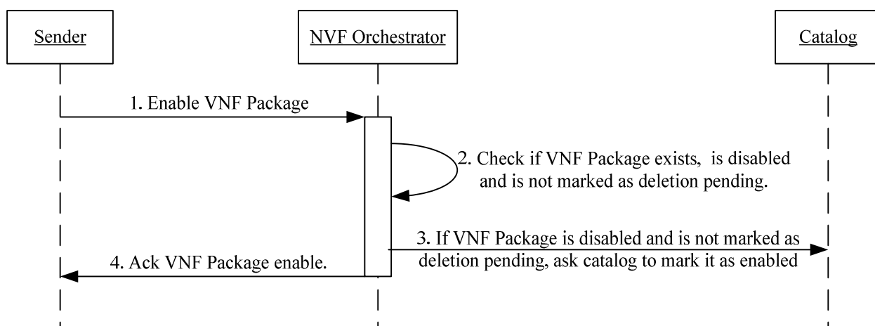
Figure B.4: Enable VNF Package message flow
