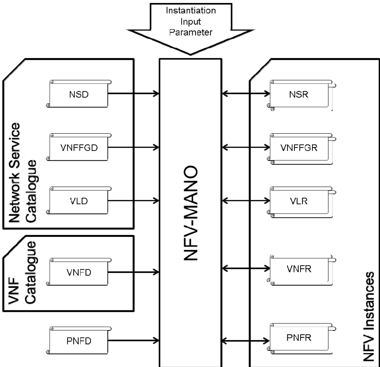
Figure 6.2: Information elements in different context
