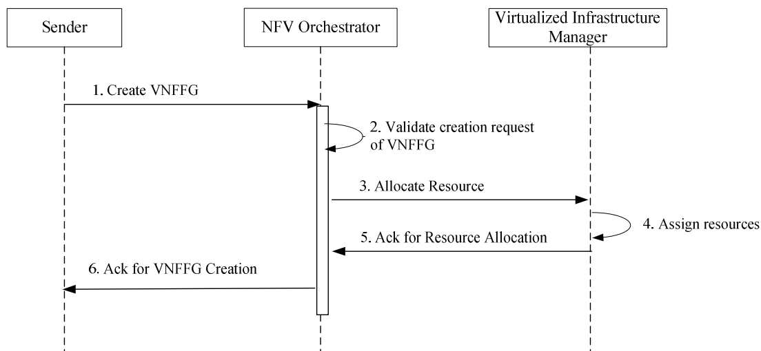
Figure C.14: VNFFG creation message flow
