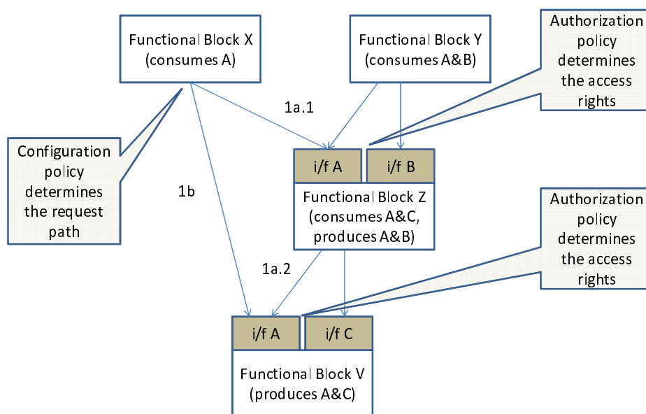
Figure 5.4: Interface concept in a Producer-Consumer paradigm
