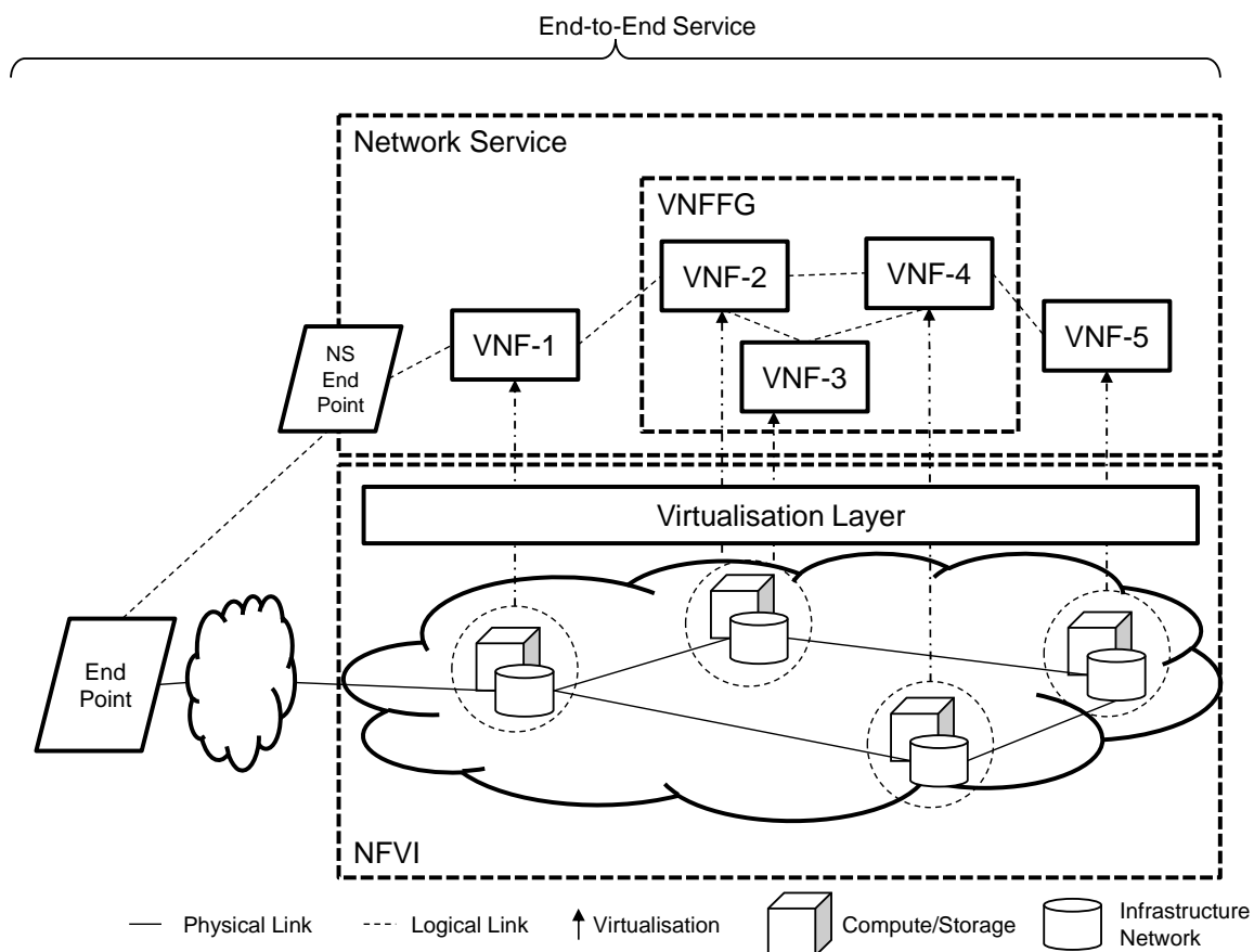
Figure 6.6: Example of a Network Service as part of an end-to-end service with VNFs and a forwarding graph
