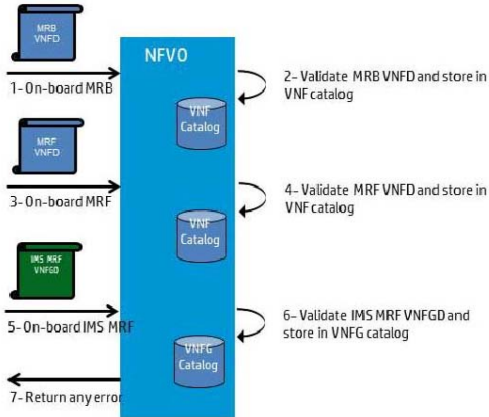
Figure A.3: IMS MRF VNF Forwarding Graph on-boarding
