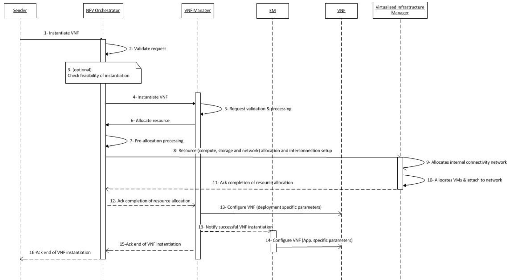
Figure B.9: VNF instantiation message flow
