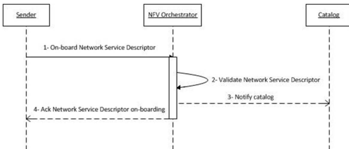
Figure C.2: Network Service Descriptor on-boarding message flow
