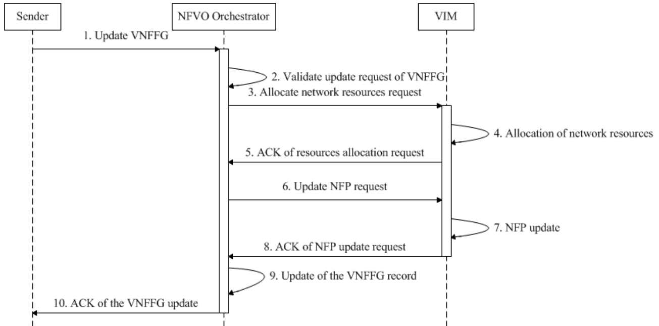
Figure C.15: VNFFG update message flow
