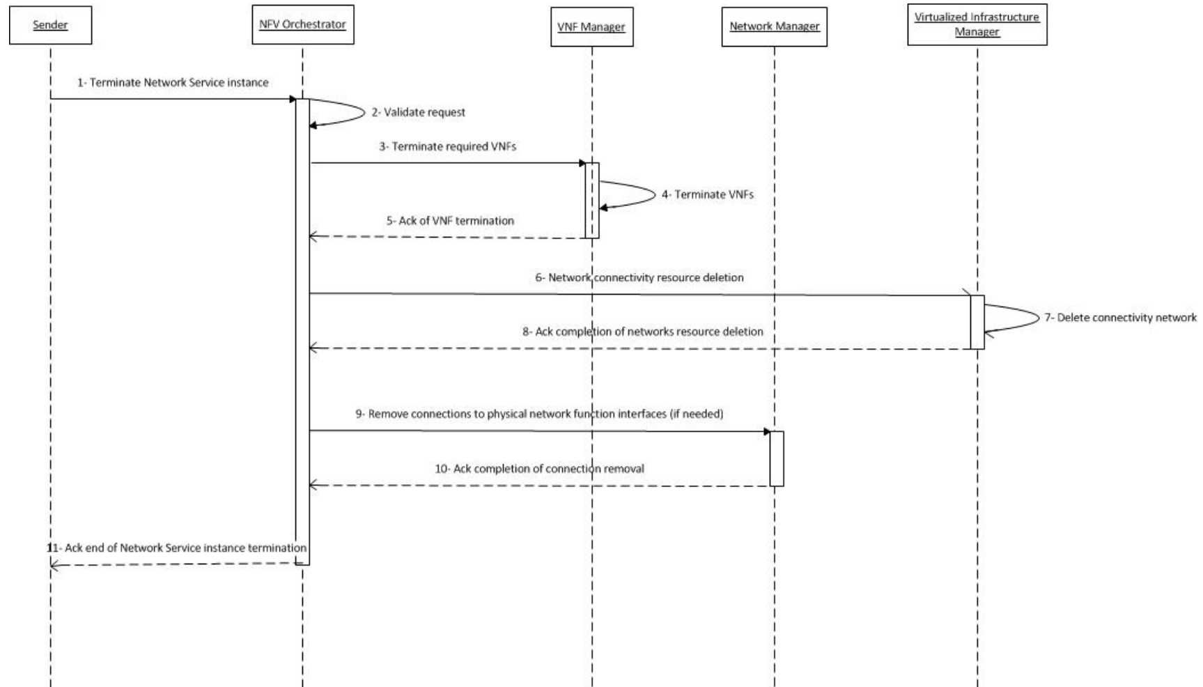
Figure C.13: Network Service termination message flow
