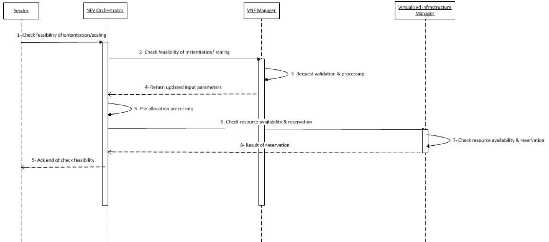
Figure B.8: VNF check feasibility message flow
