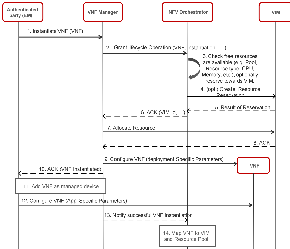
Figure B.10: VNF Instantiation from EM flow
