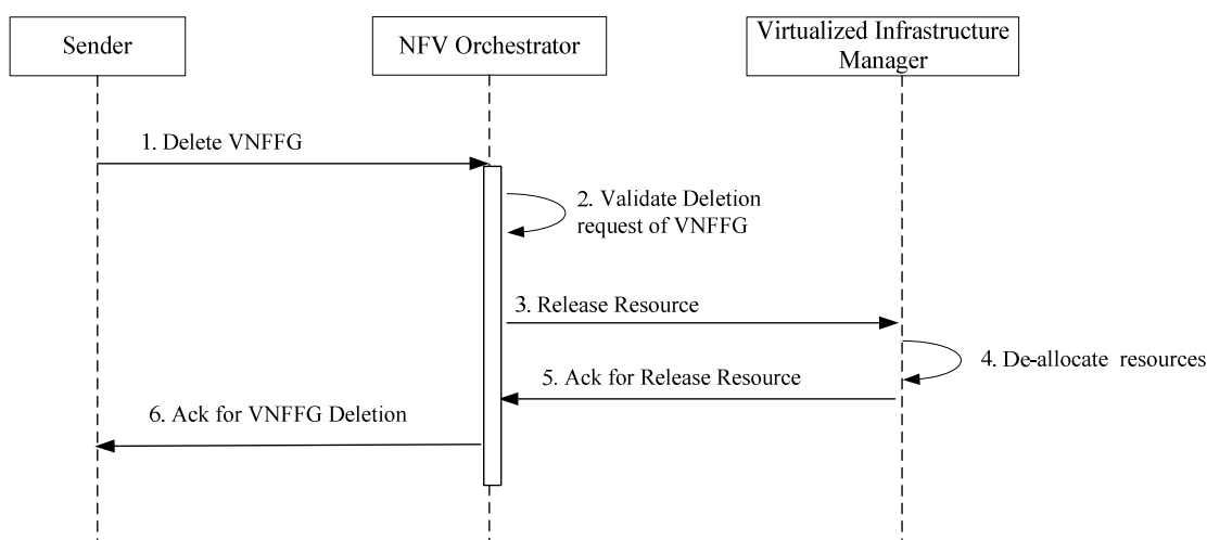
Figure C.17: VNFFG delete message flow
