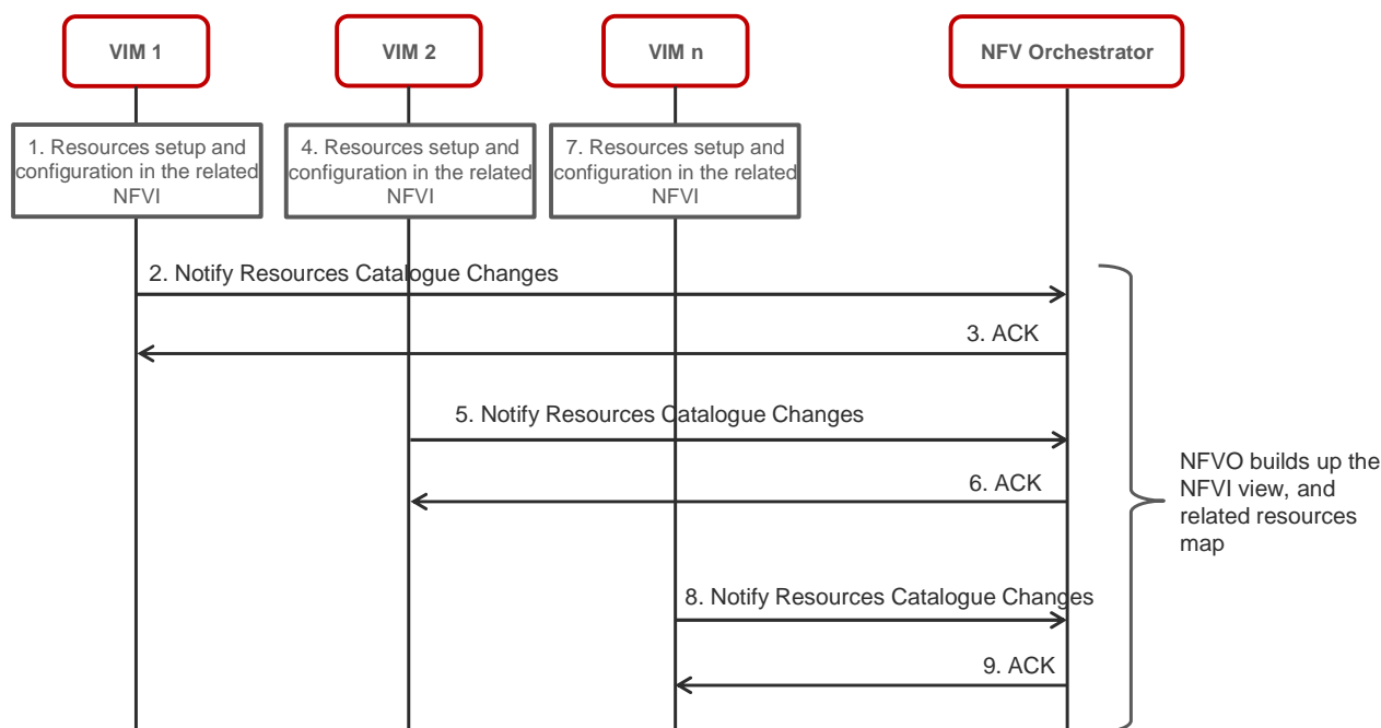
Figure D.1: NFVI-PoP setup and configuration flow
