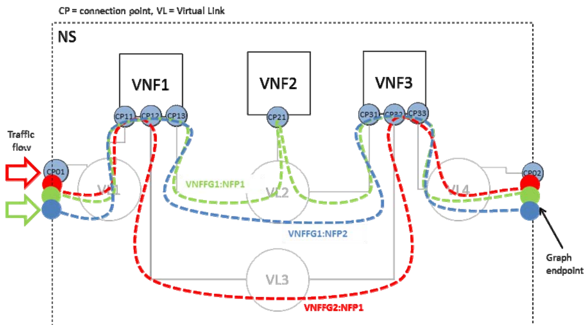
Figure 6.5: Network Service with two VNFFGs with different NFPs
