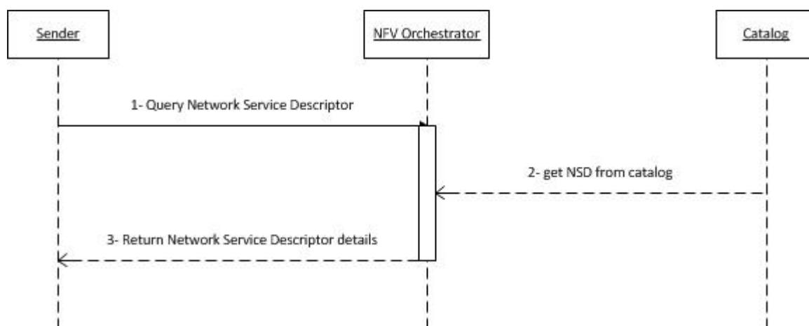
Figure C.6: Network Service Descriptor query message flow
