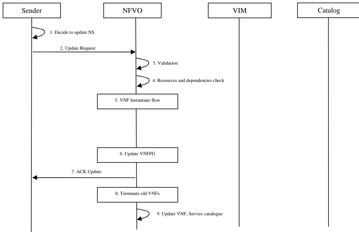
Figure C.12: NS instance update due to VNF instance modification flow
