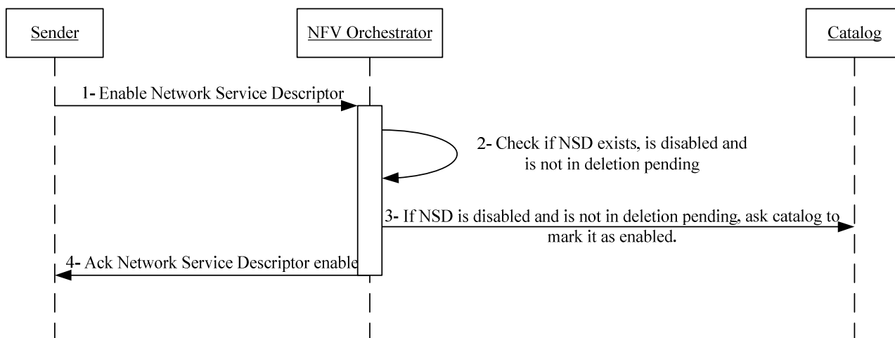
Figure C4: Network Service Descriptor enable message flow
