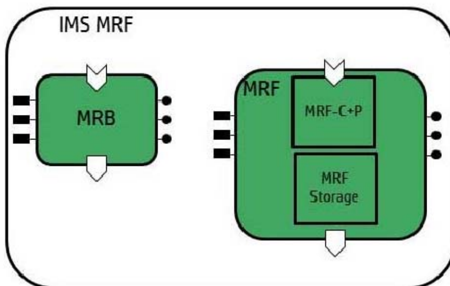
Figure A.1: IMS MRF VNF Forwarding Graph and VNFs
