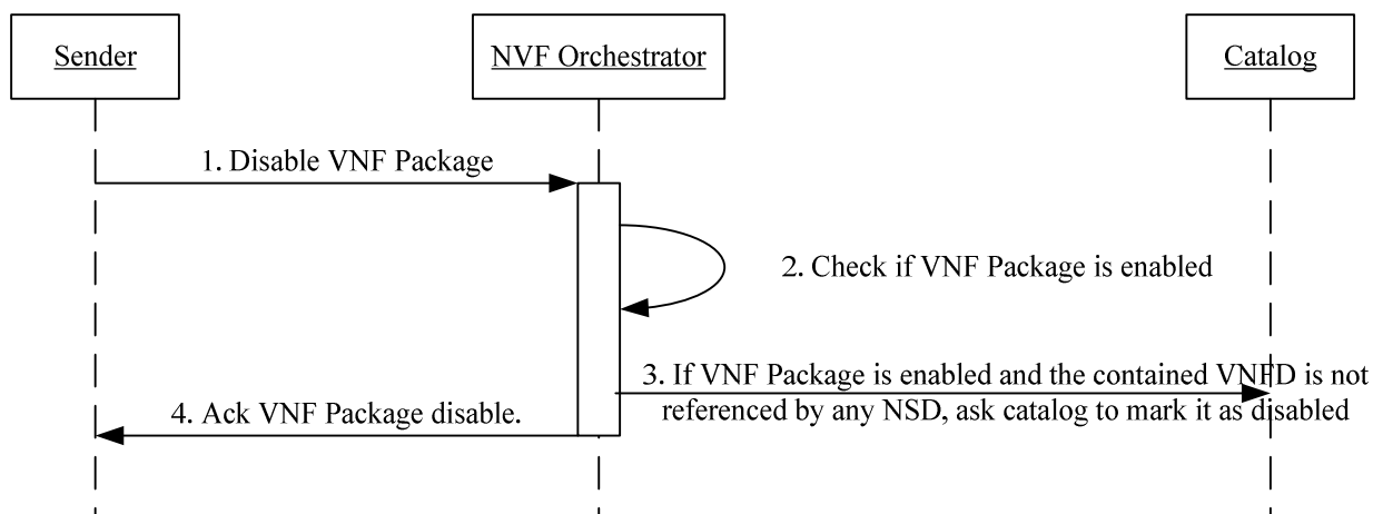
Figure B.3: Disable VNF Package message flow
