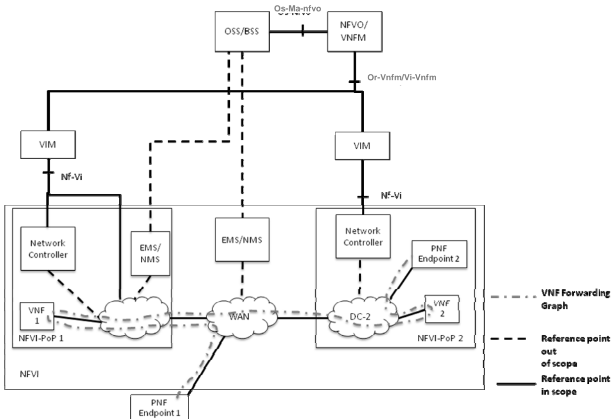
Figure 5.3: EMS/NMS for the NFVI network
