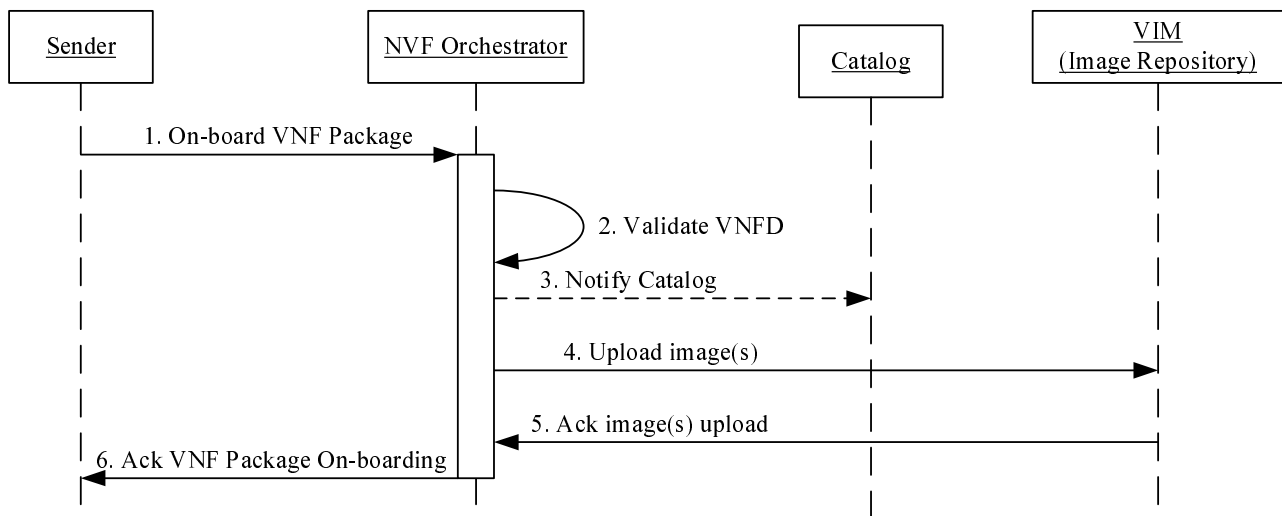
Figure B.2: VNF Package on-boarding message flow
