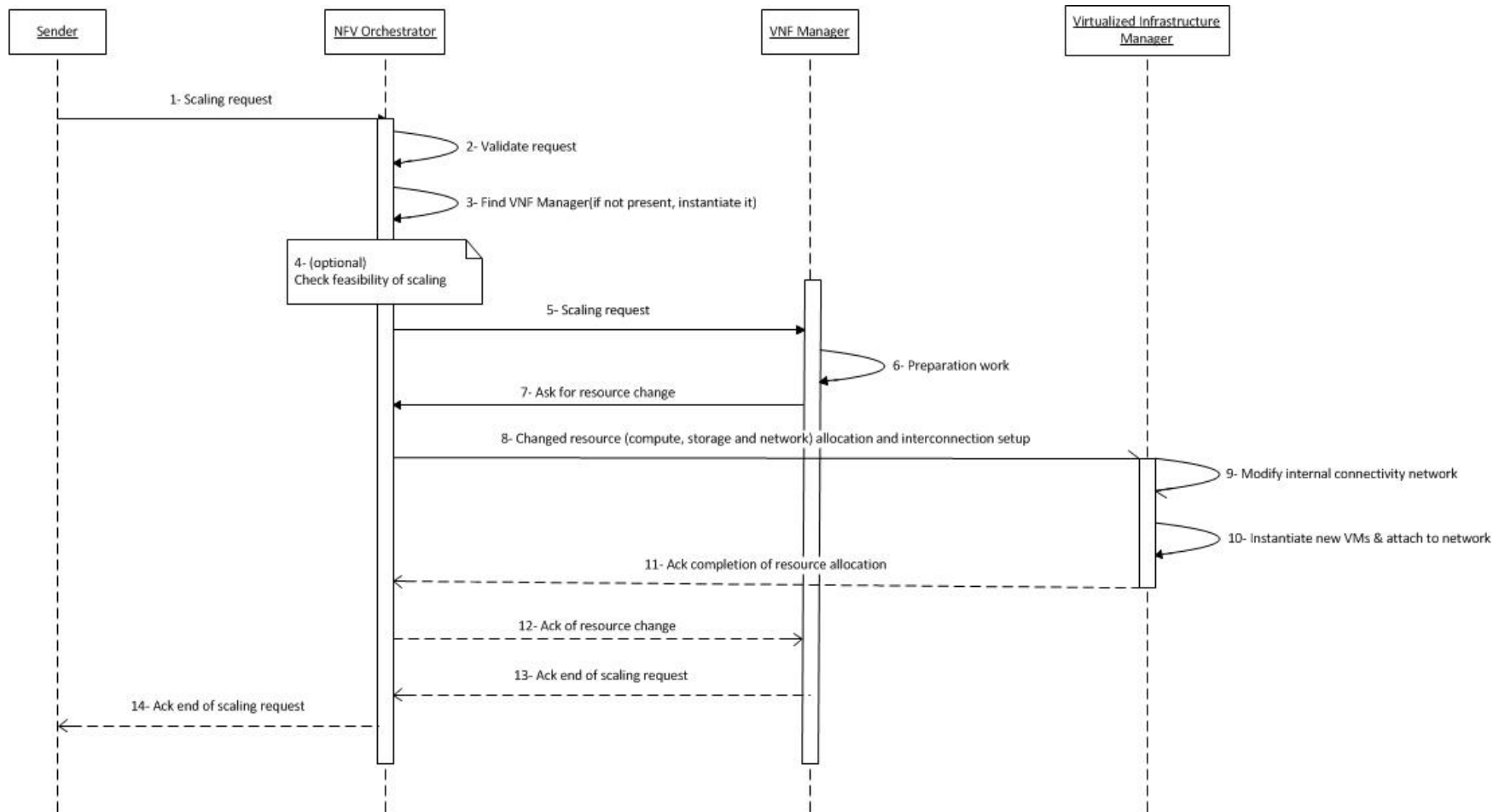
Figure B.12: VNF instance scaling message flow
