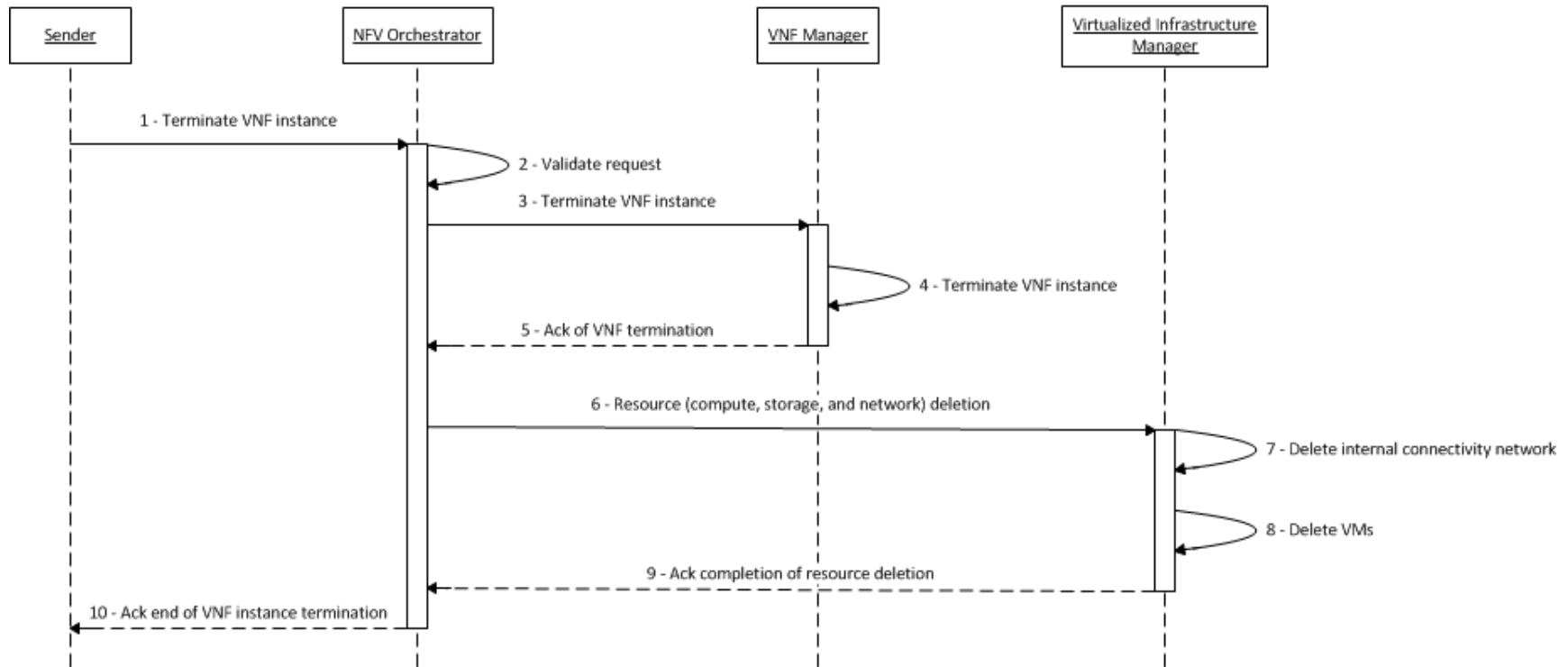
Figure B.17: VNF instance termination message flow
