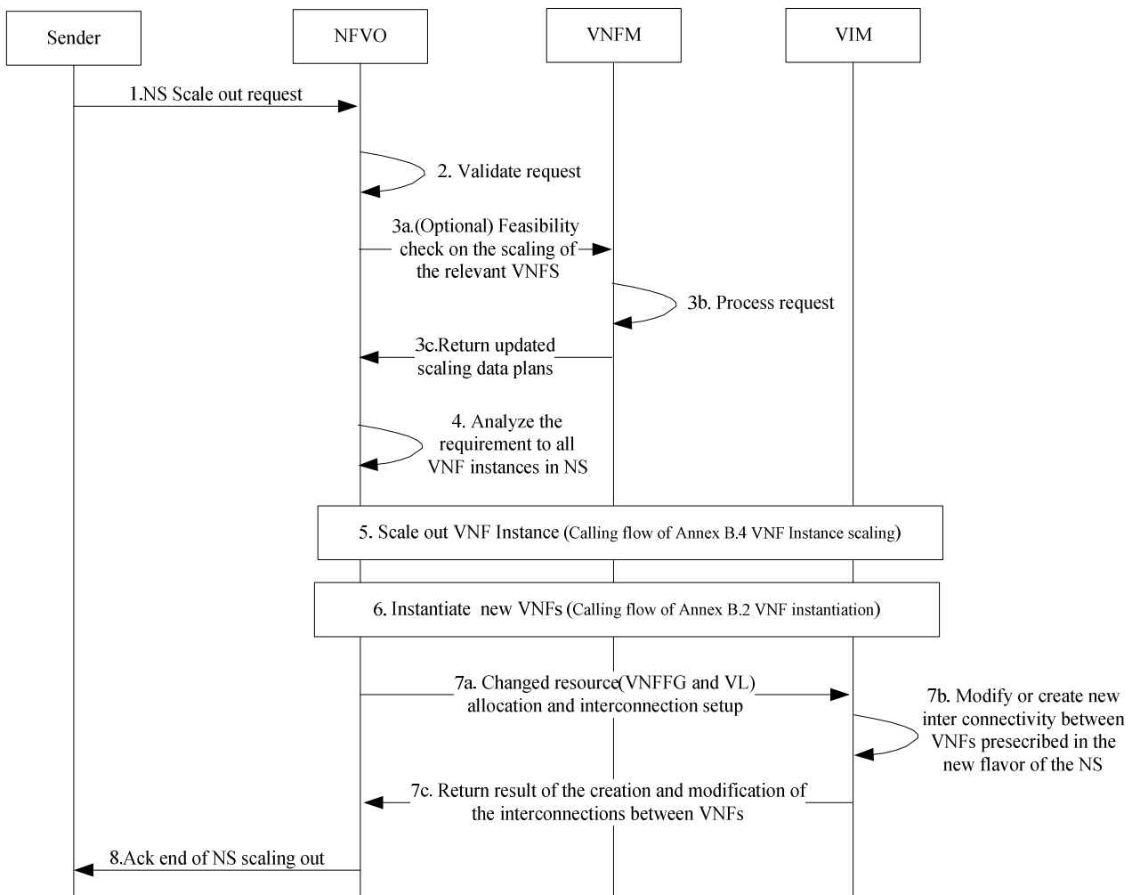
Figure C.9: Network Service scaling out message flow
