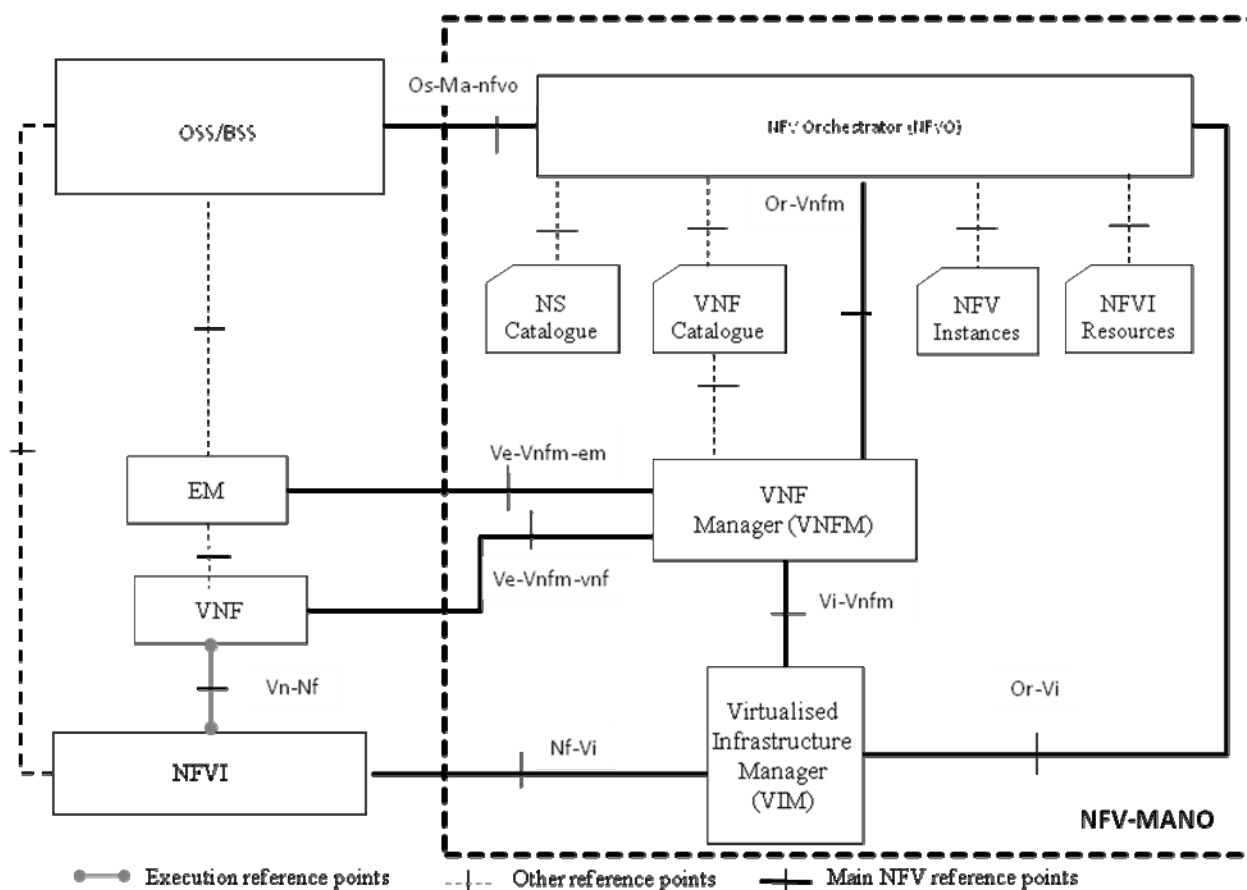
Figure 5.1: The NFV-MANO architectural framework with reference points
