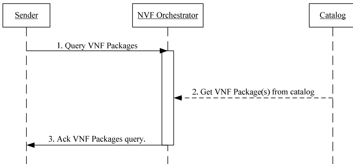
Figure B.6: VNF Package query message flow
