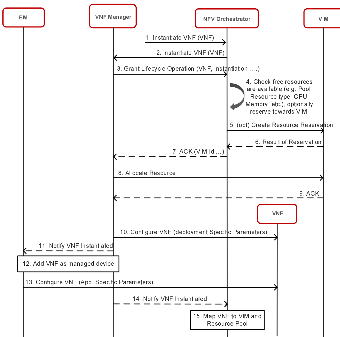
Figure B.11: VNF instantiation from NFVO flow
