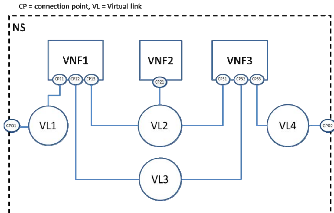
Figure 6.3: Network connection topology of a Network Service using VNFs, VLs, and Connection Points
