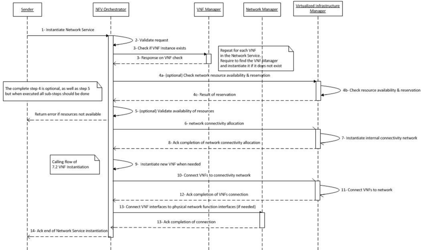
Figure C.8: Network Service instantiation message flow
