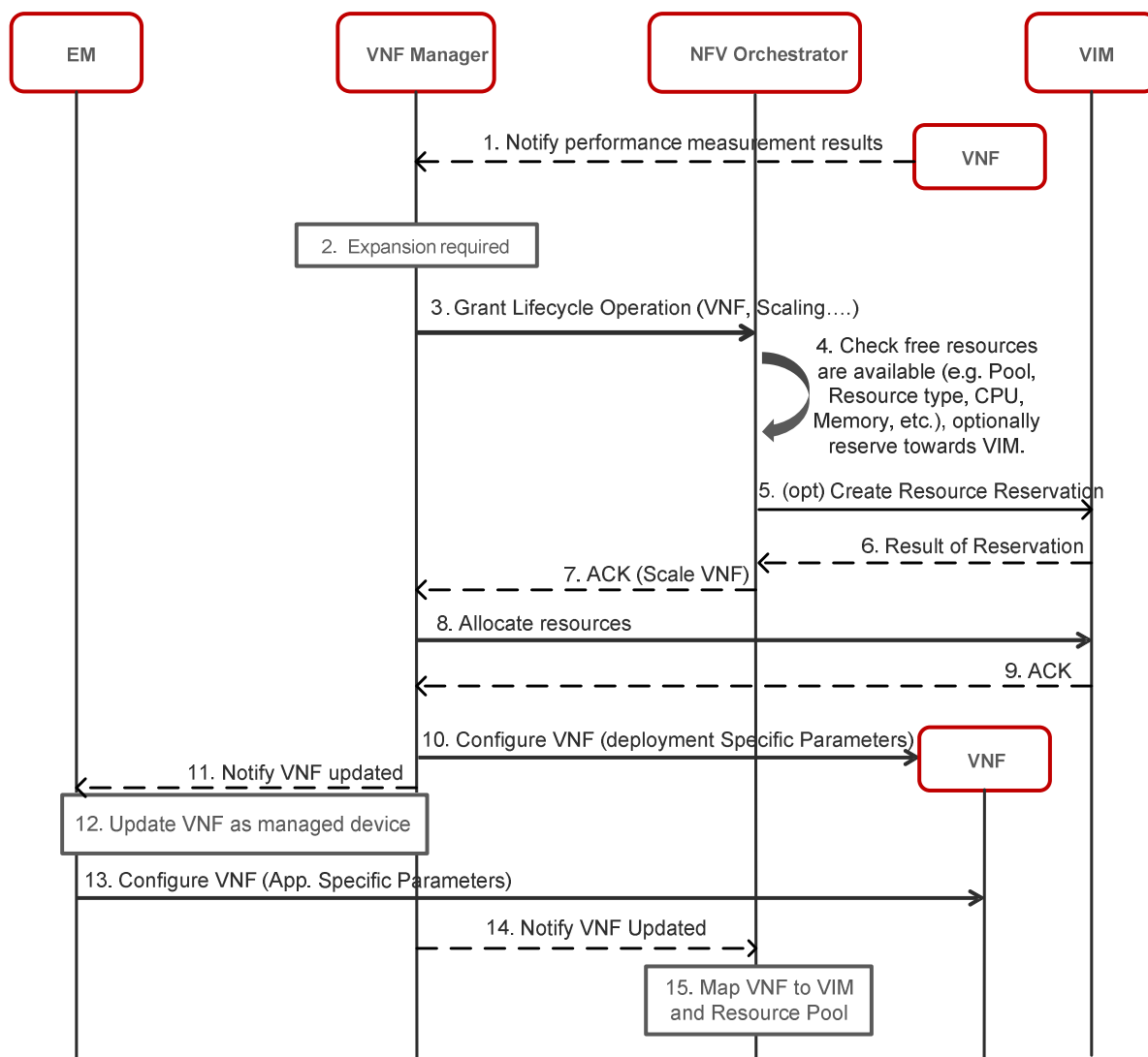
Figure B.13: Automatic VNF expansion flow triggered by VNF performance measurement results
