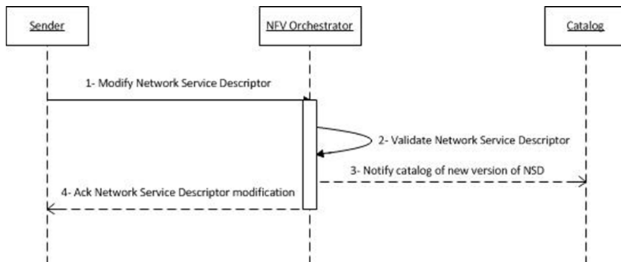
Figure C.5: Network Service Descriptor update message flow
