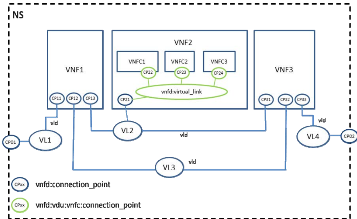
Figure 6.4: Relationships between internal and external Virtual Links
