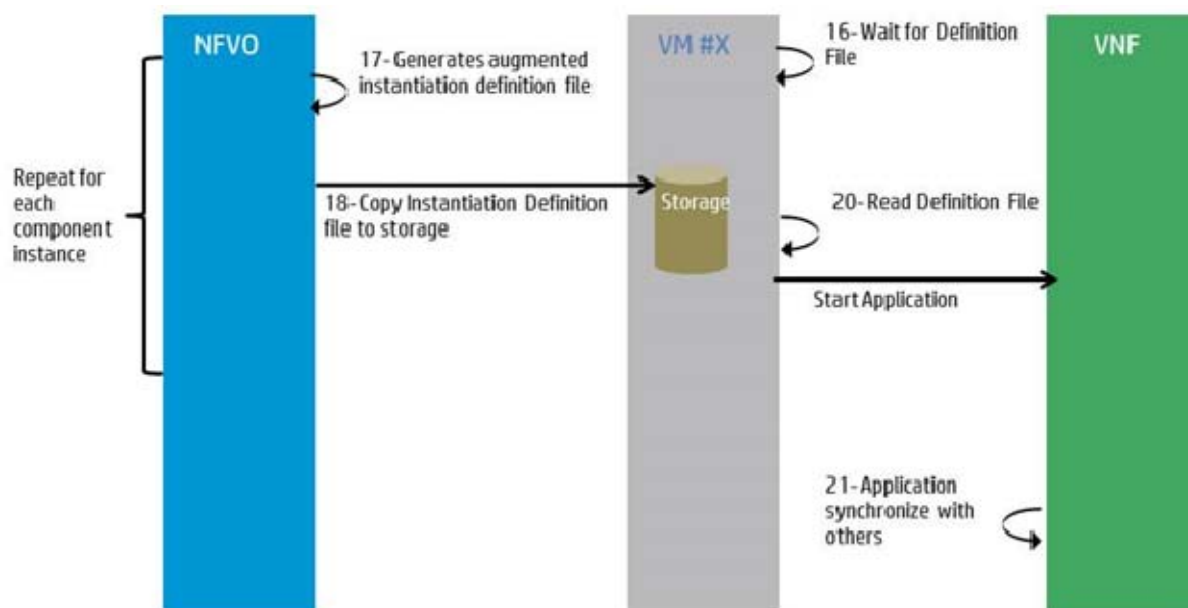
Figure A.7: IMS MRF Deployment Sequence Diagram - Configuration phase
