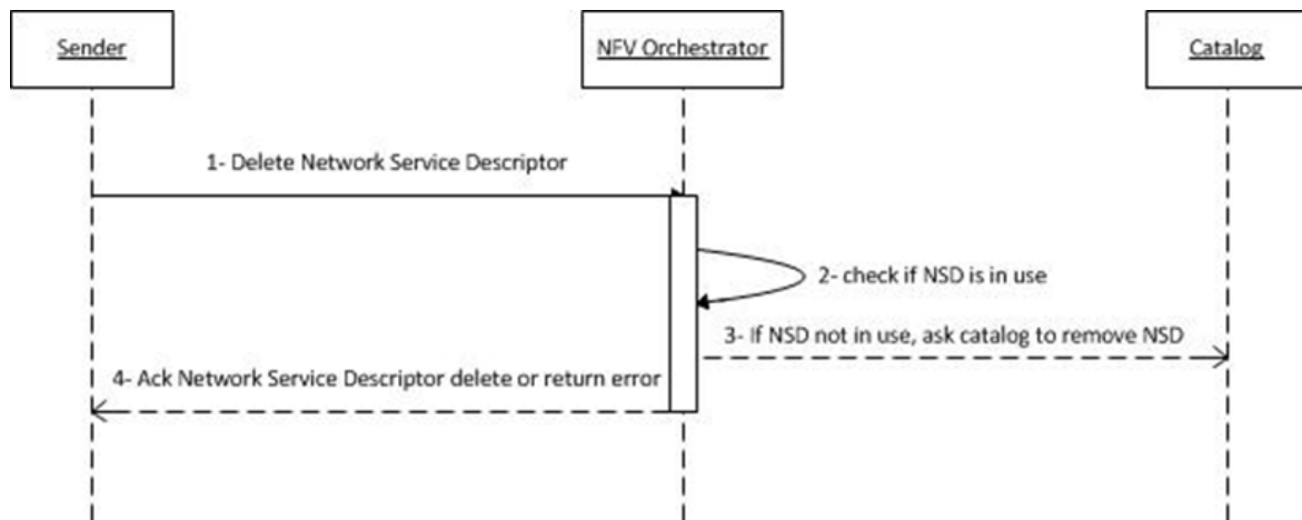
Figure C.7: Network Service Descriptor deletion message flow
